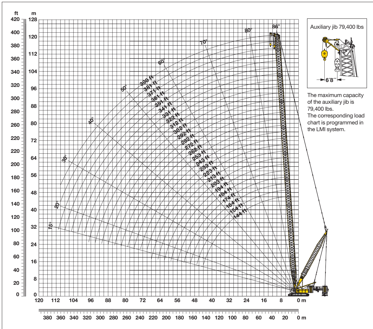
Configuration for boom lengths between 144 ft and 390 ft
