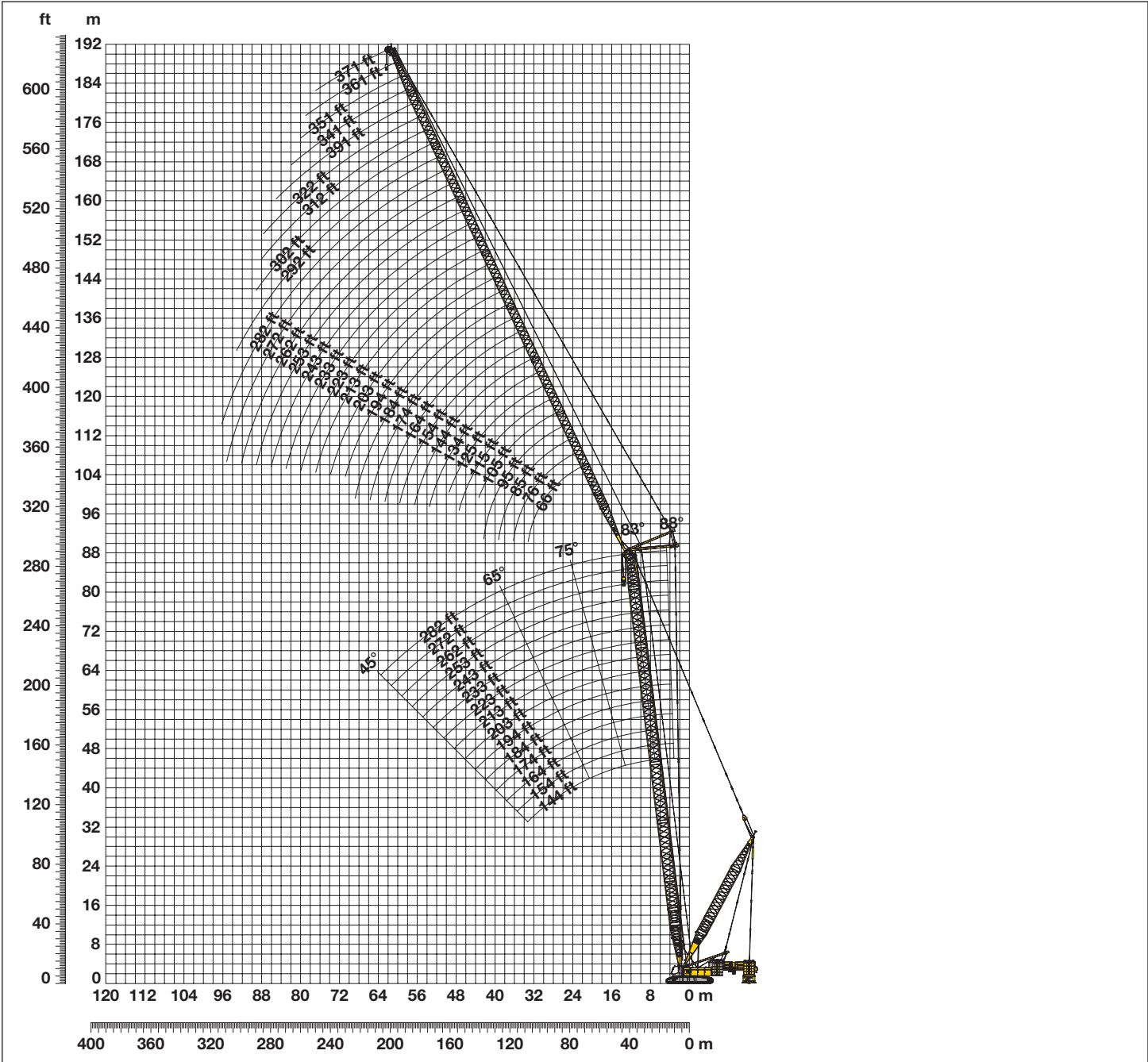
Boom configuration for main boom lengths (144 ft - 282 ft) – see table 1 on page 4 Jib configuration for jib lengths (66 ft - 371 ft)
