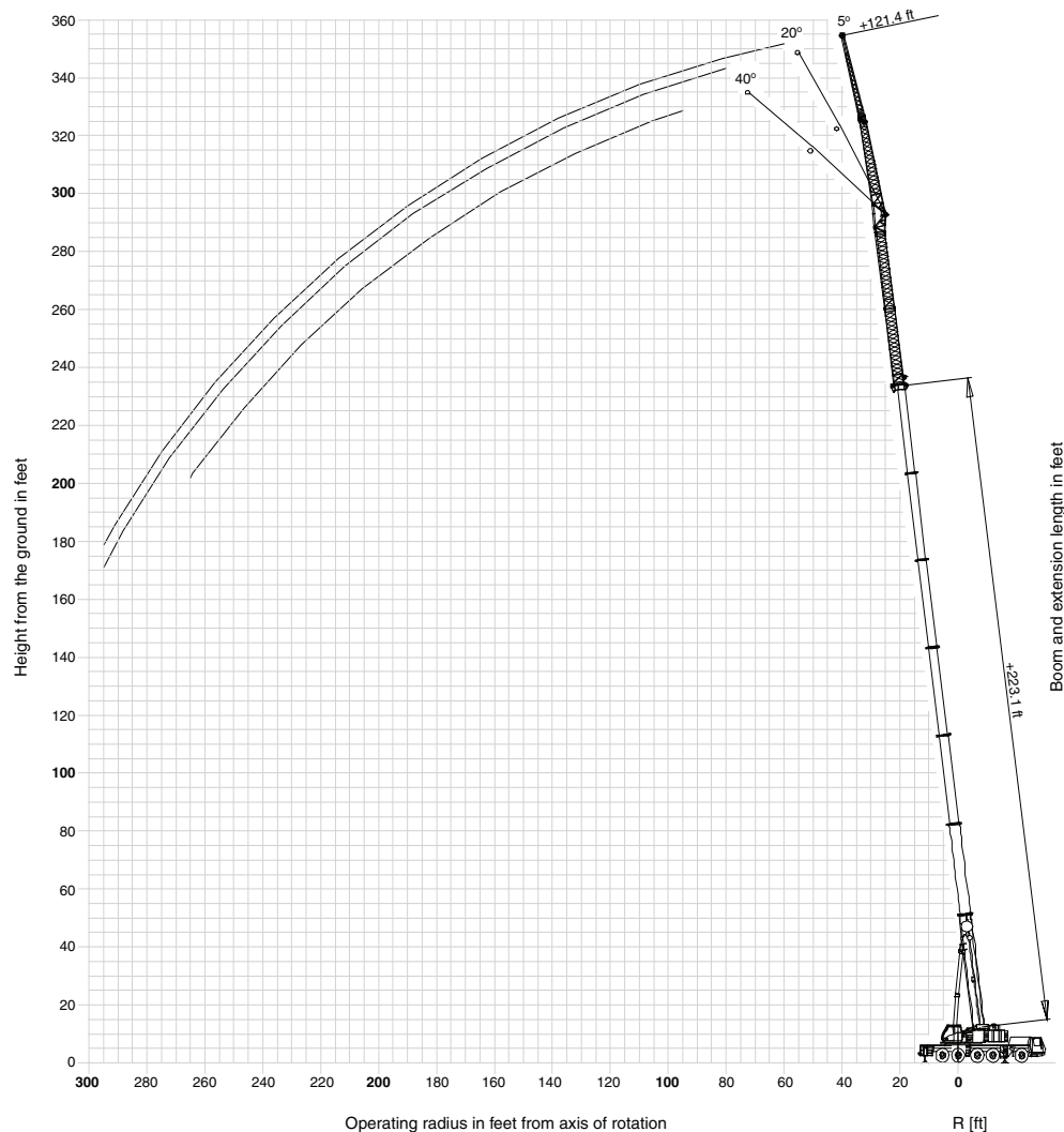
223' Main Boom, 68.9' Swingaway and 2 x 26 ft. Inserts
