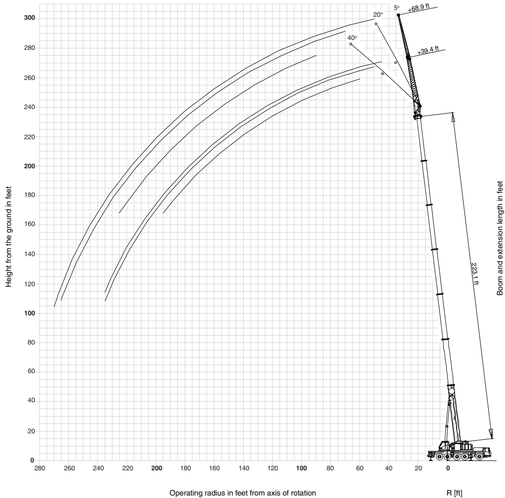
223' Main Boom with 39.4 ft. and 68.9 ft. Swingaway
