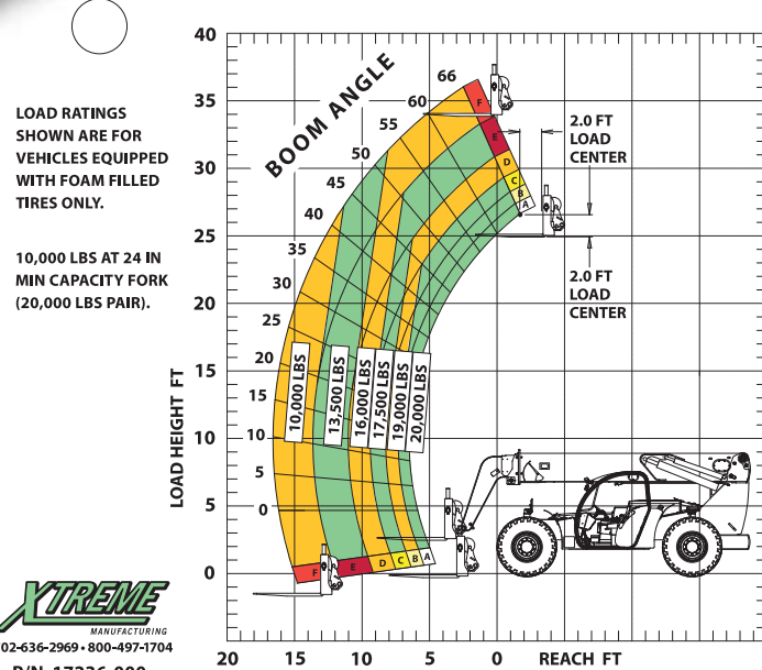
XR2034 LOAD CHART - STANDARD CARRIAGE
