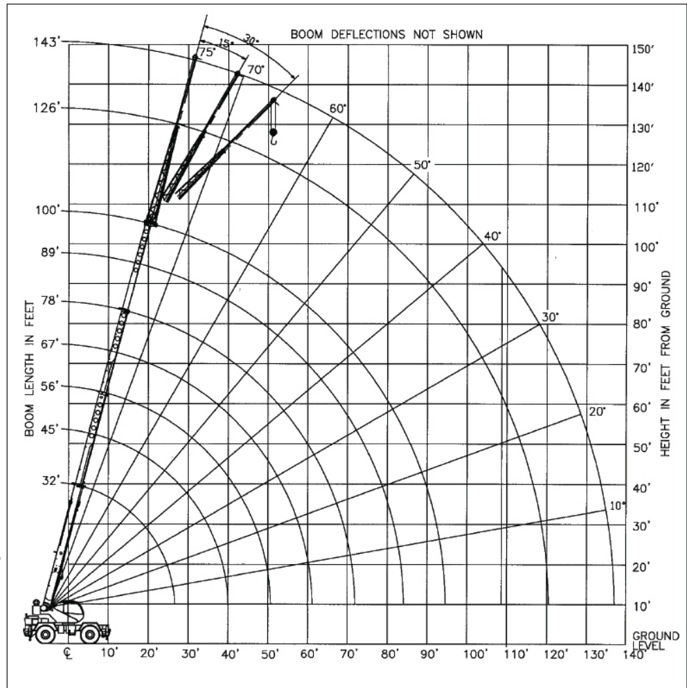
Range Diagram (32' - 100' boom)
