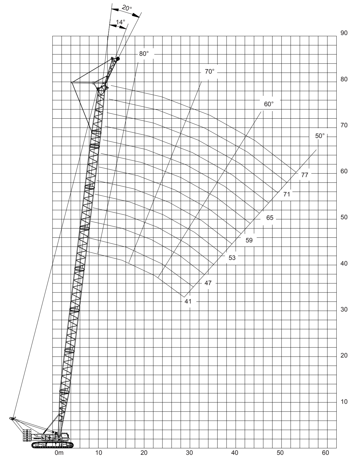
Heavy Fixed Jib Lifting Height Curve
