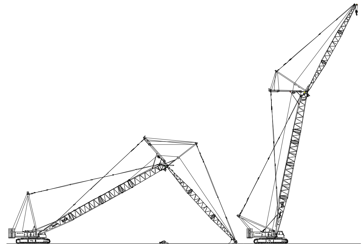
Boom and lifting
