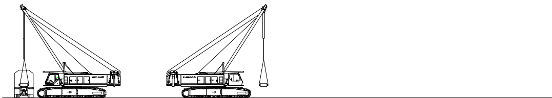
Unloading and assembling of vehicle body ballast weight
