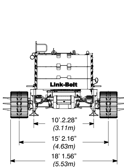
Extended Gauge
