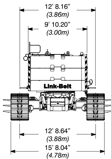
Intermediate Gauge
