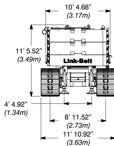
Retracted Gauge
