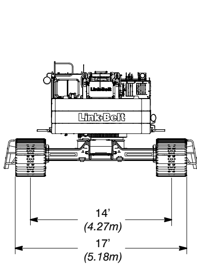
Extended Gauge
