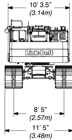
Retracted Gauge
