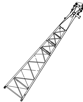
25' Angle Boom Top With Pile Driver Lead Adapter
