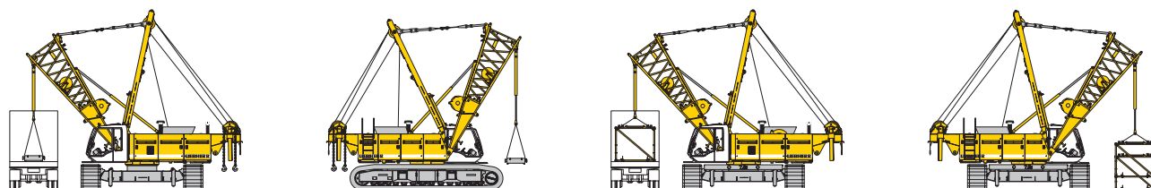
Unloading and assembly of carbody counterweight
