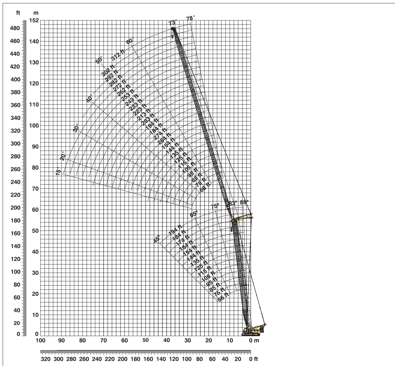
Boom configuration for main boom lengths (66 ft - 194 ft) – see table 1 on page 10 Jib configuration for jib lengths (66 ft - 312 ft)
