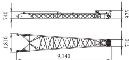
Rear Strut (Luffing Jib) Weight: 1,510 kg
