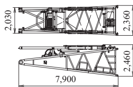
70 t Hook Weight: 1,200 kg
