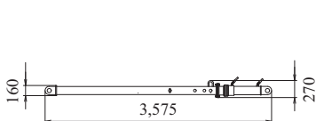
Strut Backstop (Luffing Jib) Weight: 180 kg
