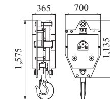
35 t Hook Weight: 900 kg
