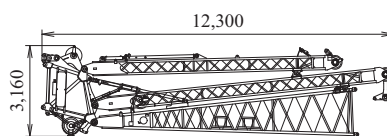
Luffing Boom Tip Assembly Weight: 6,730 kg
