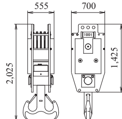
100 t Hook Weight: 1,800 kg
