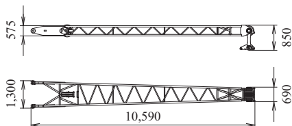
Front Strut (Luffing Jib) Weight: 1,410 kg
