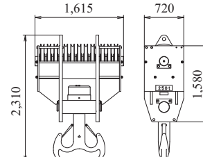
250 t Hook Weight: 4,200 kg
