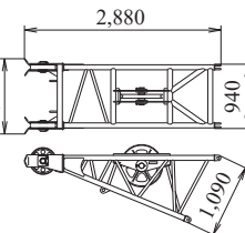
Jib Upper Spreader (for Luffing) Weight: 260 kg
