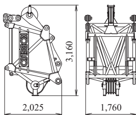
3.0 m Luffing Jib Insert Weight: 320 kg
