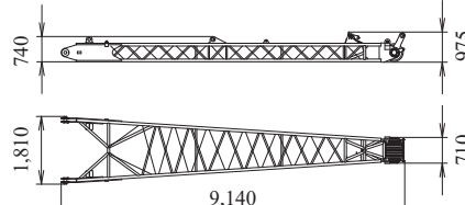
Rear Strut (Luffing Jib) Weight: 1,510 kg
