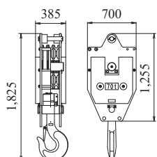
70 t Hook Weight: 1,200 kg
