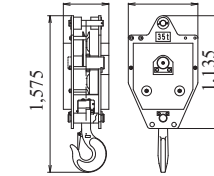
250 t Hook Weight: 4,200 kg
