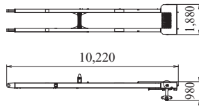
Mast Weight: 3,320 kg
