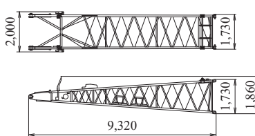
Luffing Jib Base Weight: 1,470 kg
