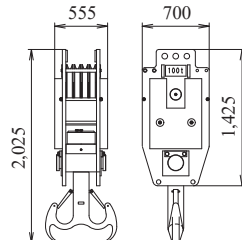
100 t Hook Weight: 1,800 kg
