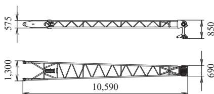
Front Strut (Luffing Jib) Weight: 1,410 kg
