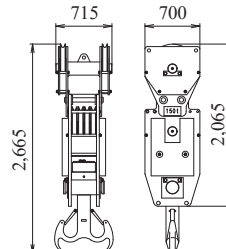
150 t Hook Weight: 2,300 kg
