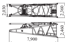
Boom Base (with Winch) Weight: 6,810 kg
