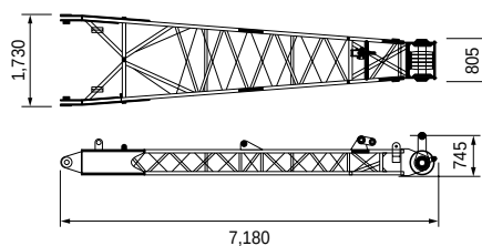
Rear Strut (Luffing Jib) Weight: 1,090 kg
