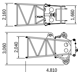
Luffing Jib Base Weight: 1,140 kg
