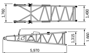
Luffing Jib Base Weight: 1,140 kg
