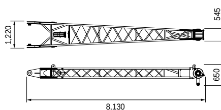
Front Strut (Luffing Jib) Weight: 1,000 kg
