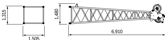
Luffing Jib Top Weight: 1,170 kg
