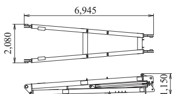
Jib Strut (Luffing Jib) Weight: 2,010 kg
