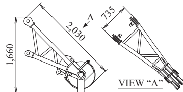
Auxiliary Sheave (for Crane) Weight: 300 kg
