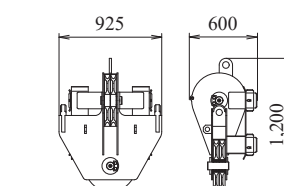
70 t Hook Weight: 1,200 kg
