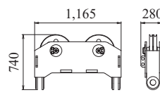
Lower Spreader (for Crane) Weight: 300 kg
