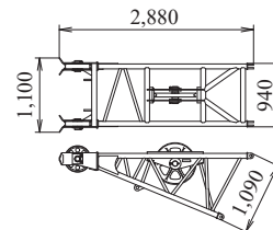
Jib Upper Spreader (for Luffing) Weight: 260 kg
