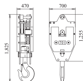
70 t Hook Weight: 1,200 kg
