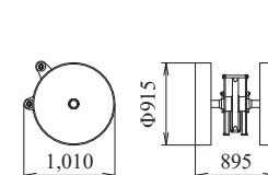
Auxiliary Sheave (for Luffing) Weight: 380 kg
