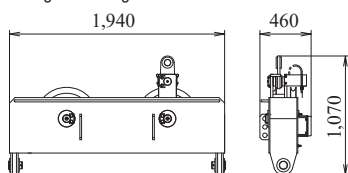
Jib Lower Spreader (for Luffing) Weight: 405 kg
