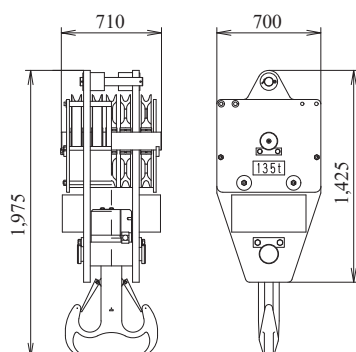
135 t Hook Weight: 1,700 kg
