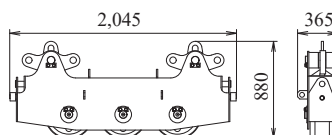
Upper Spreader (for Crane) Weight: 485 kg
