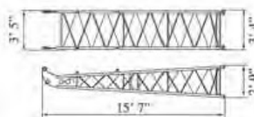
Jib Base (for Crane) Weight: 465 lbs
