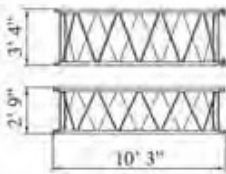
10 ft Insert Jib Weight: 245 lbs
