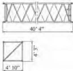
40 ft Insert Jib Weight: 2,115 lbs
