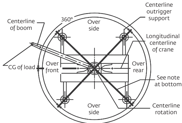
Diagram for lifting on outriggers
