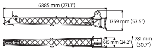
Boom extension - 6,5 m (21 ft 4 in)
