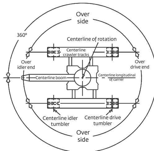
Working area diagram
