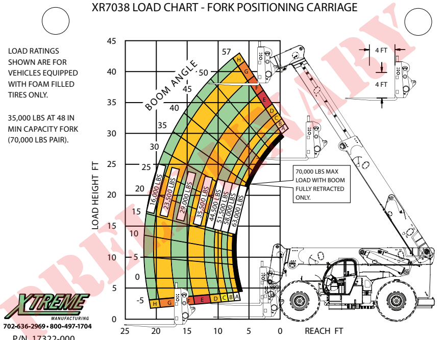
XR7038 LOAD CHART - FORK POSITIONING CARRIAGE
